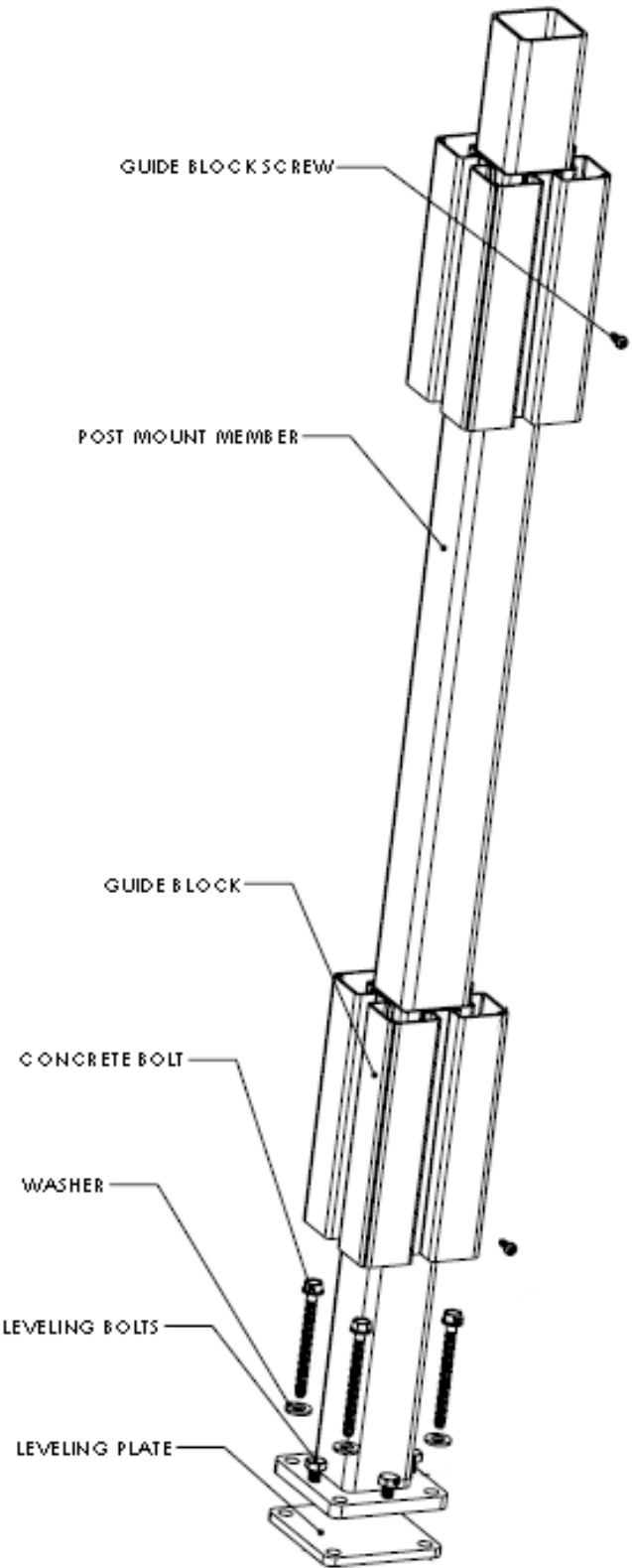
FIGURE 3—ULTRA POST
