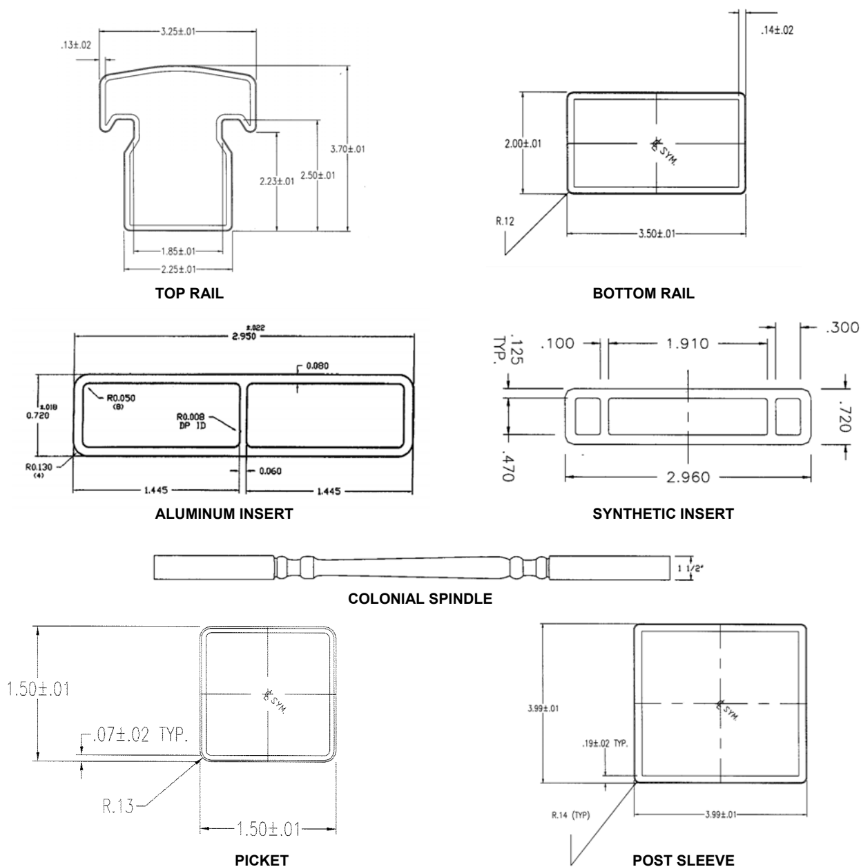
FIGURE 1—CROSS SECTIONS
