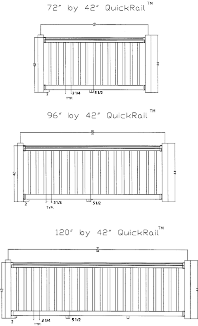
FIGURE 2—ASSEMBLIES
